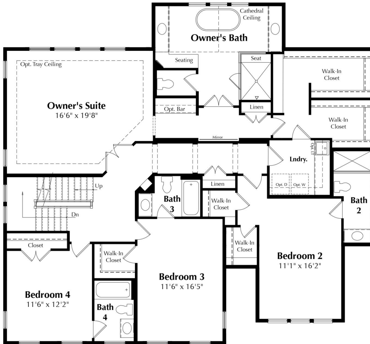
Second Level Floor Plan
