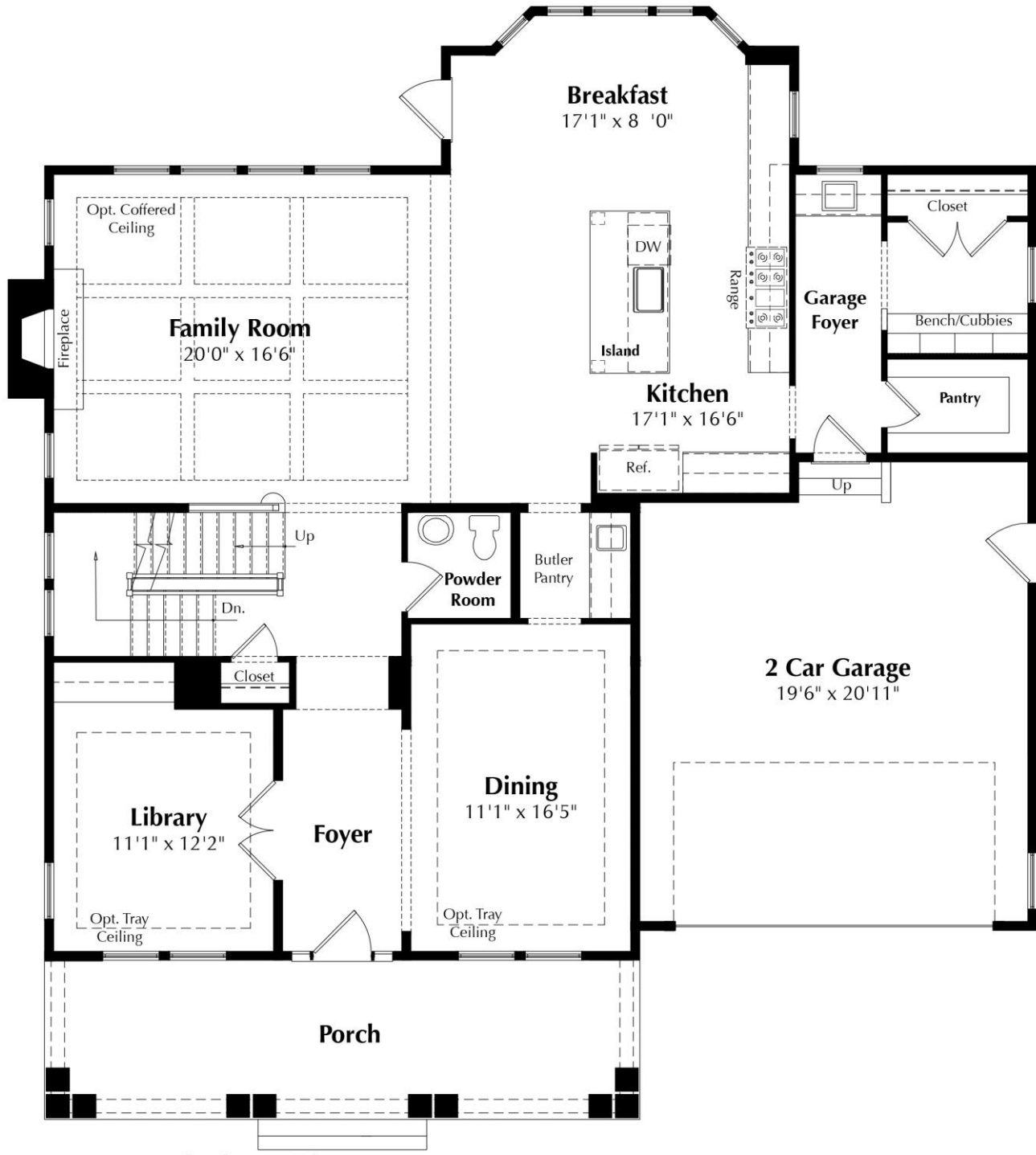
First Level Floor Plan
