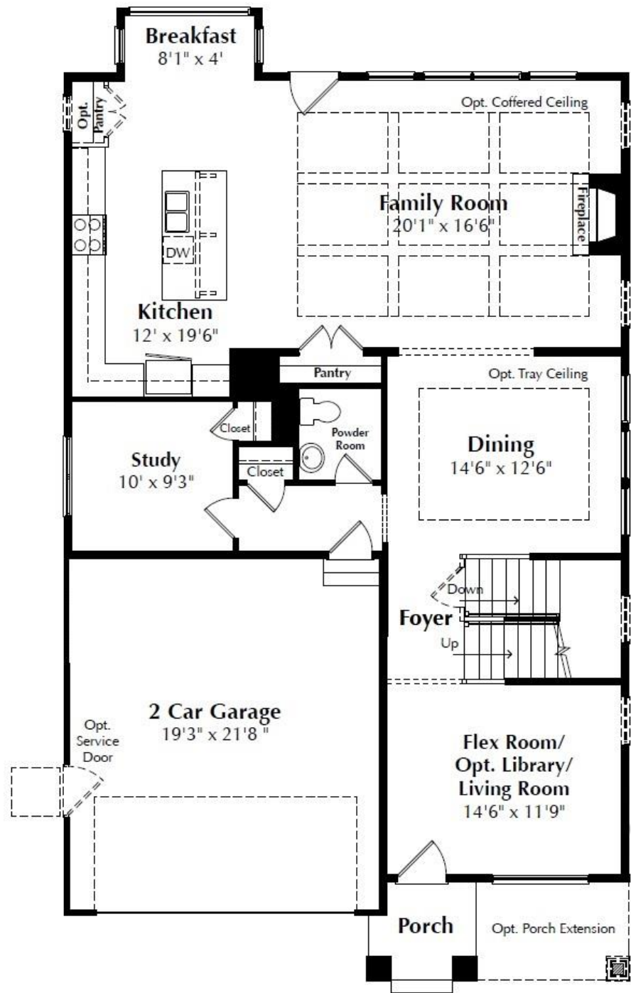
First Level Floor Plan
