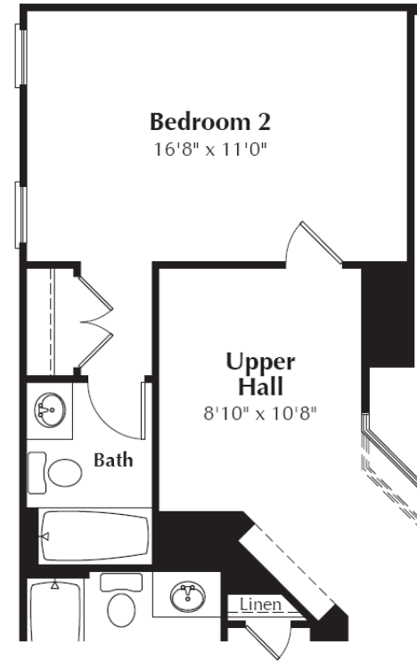
Partial Second Level Floor Plan With Optional Bedroom 2 Bath
